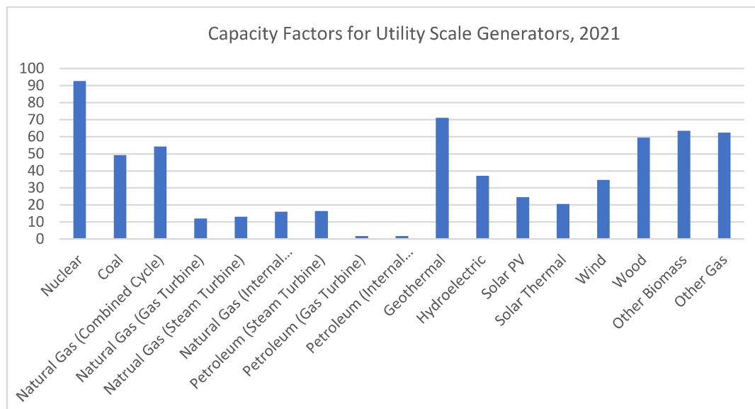
Figure 16. Capacity Factors for Utility Scale Generators.
