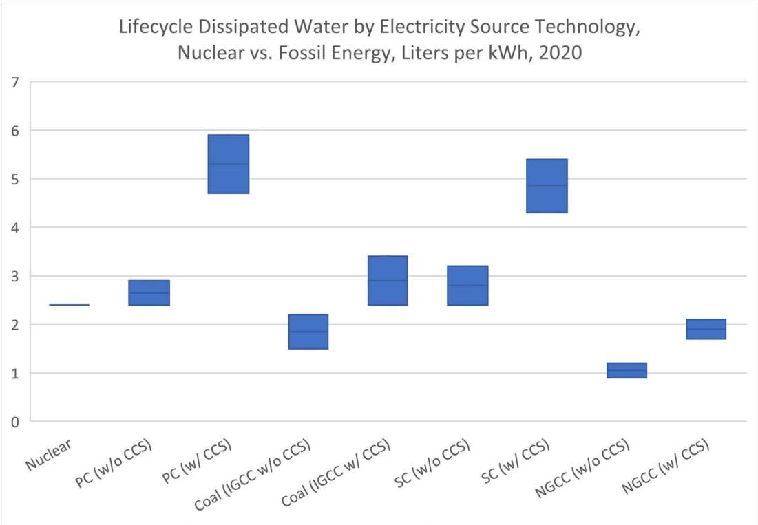
Figure 13. Lifecycle Dissipated Water by Electricity Source Technology.
