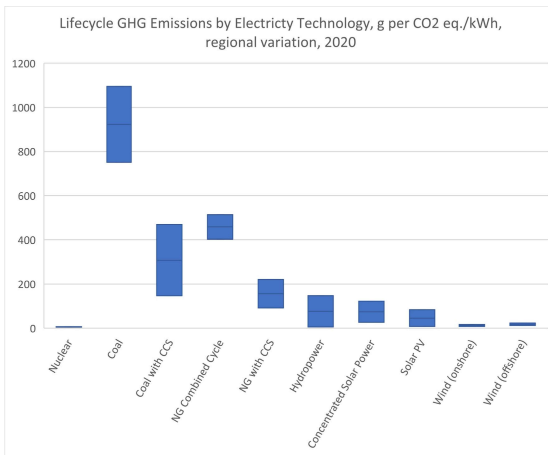
Figure 4. Lifecycle GHG Emissions by Electricity Technology.
