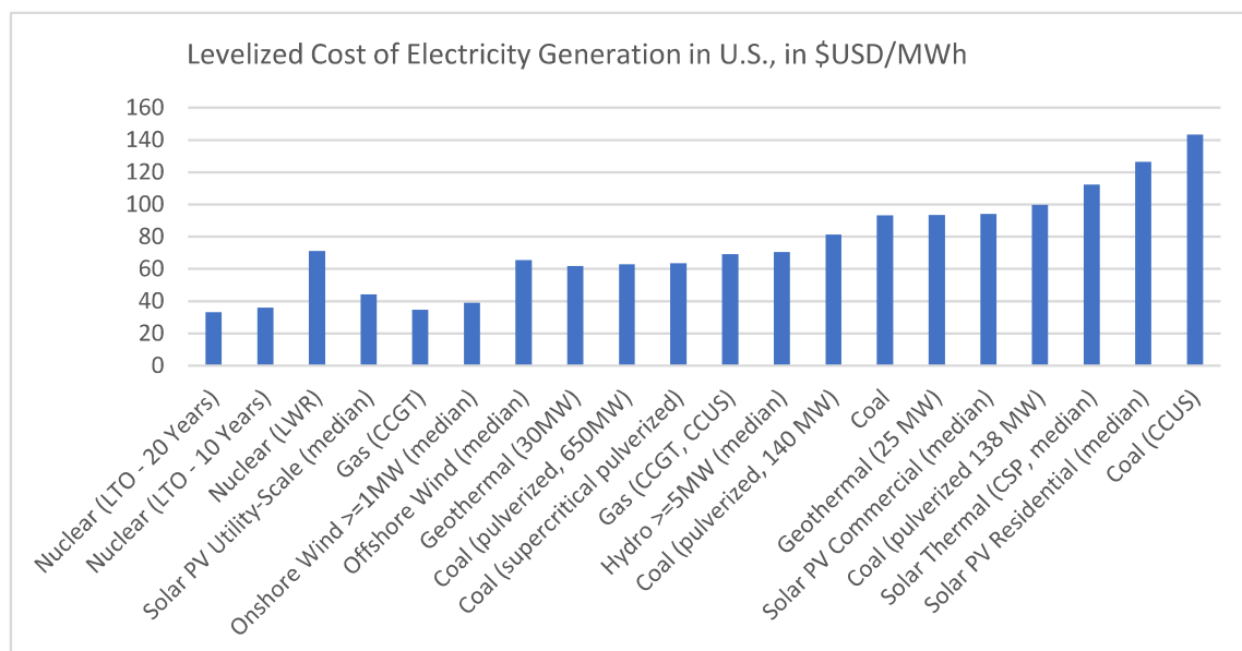
Figure 20. Levelized Cost of Electricity Generation in U.S.
