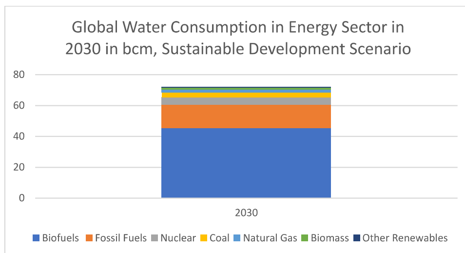
Figure 12. Global Water Consumption in Energy Sector.
