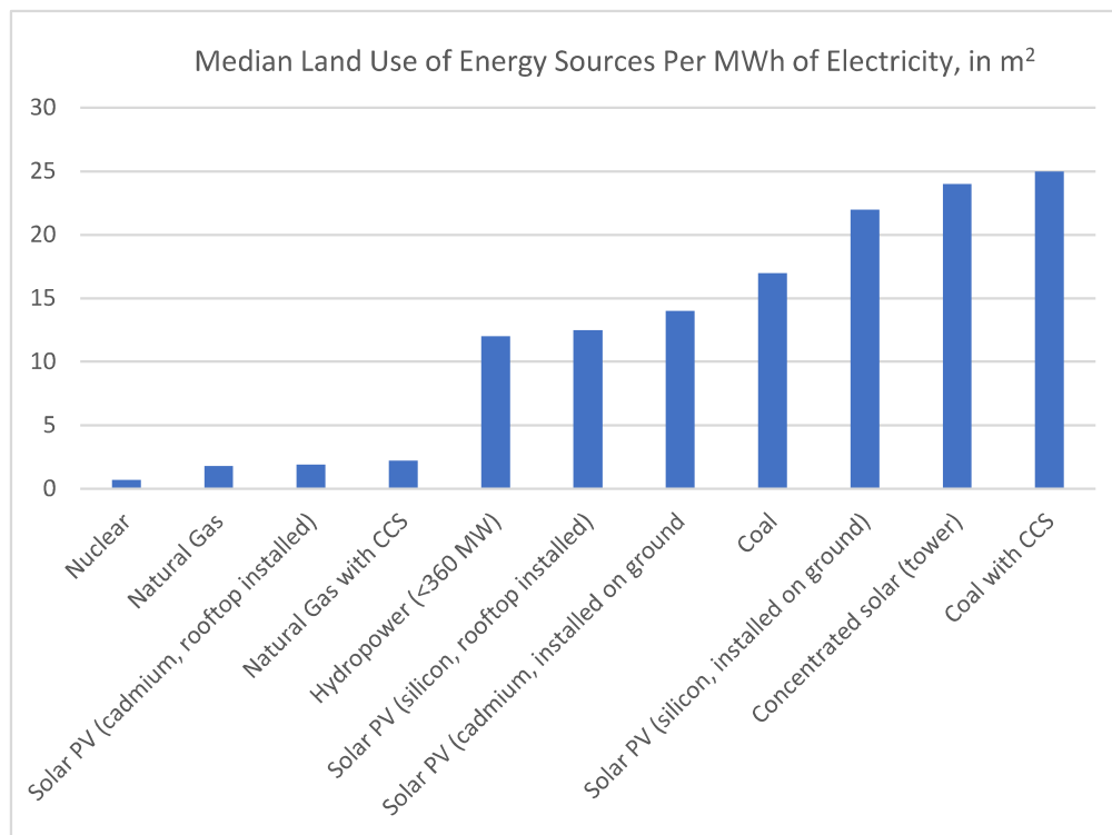
Figure 8. Median Land Use of Energy Sources.
